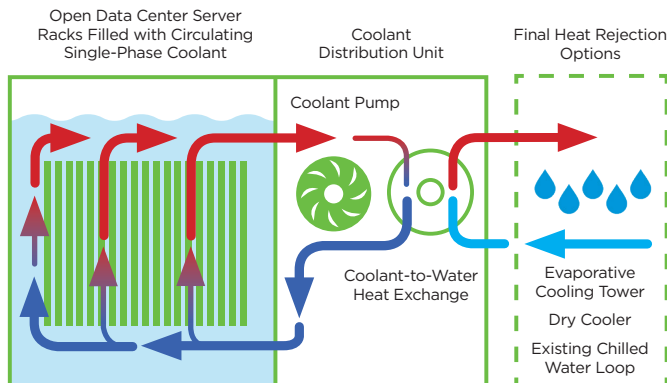
Heated Coolant Exits Top of Rack, Cycles Through the CDU and Returns to the Rack at a User-Specified Temperature.
