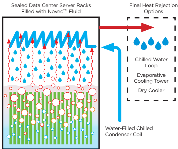
Novec Fluid Boils from Server Heat, Transforms from Liquid to Vapor and Passively Condenses Back to Liquid When It Contacts Water-Cooled Condenser Coils
