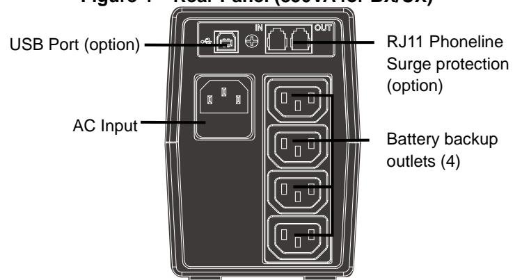
Figure 4 – Rear Panel (850VA for BX/UX)
